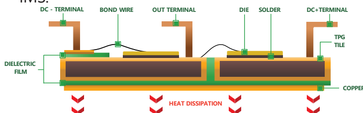
Figure-4 IMSwTPG-Based Half-Bridge Power Module
