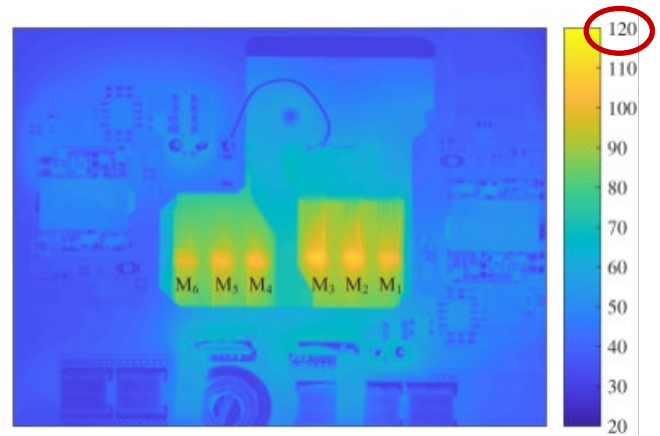
Figure-8 IMSwTPG substrate
