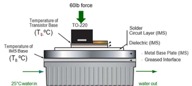
Water-cooled Heatsink
