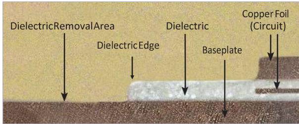
Precision laser removal of dielectric, to expose base for direct component mounting
