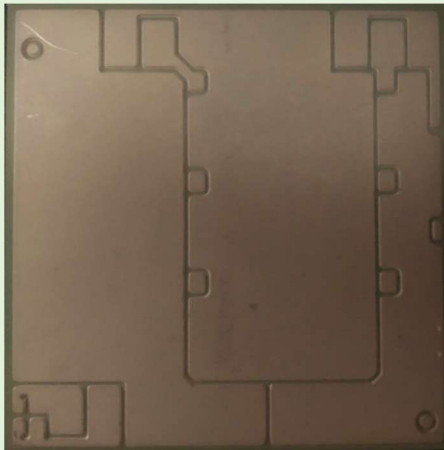
Power Module with 17oz (595μm) Circuit Copper and Copper Base
