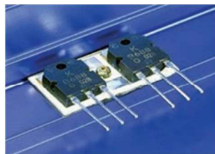
THERMAL CLAD measured junction temperature 5W= T_J 35°C
