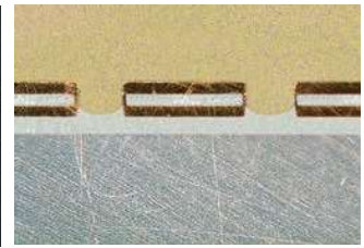
Laminated thick copper up to 5 oz. (175µm) finished on the internal layer using HT dielectric
