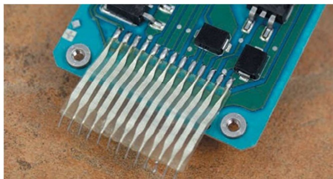
Flex tail hot bar soldered to THERMAL CLAD.
