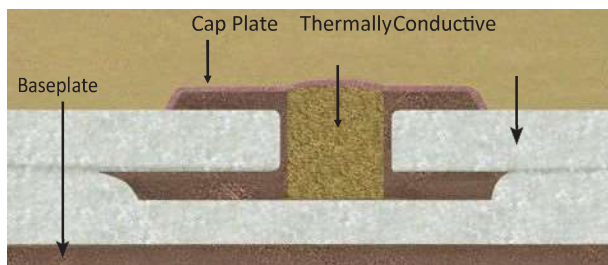
IPC type 7 Polymer Filled Via, conductive or non-conductive, with cap plating for void free component mounting
