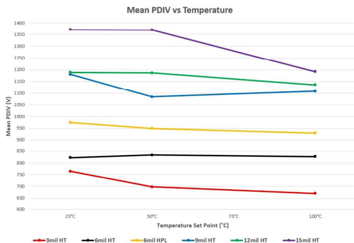
Figure-5 Mean PDIV as Function of Temperature Set Point
